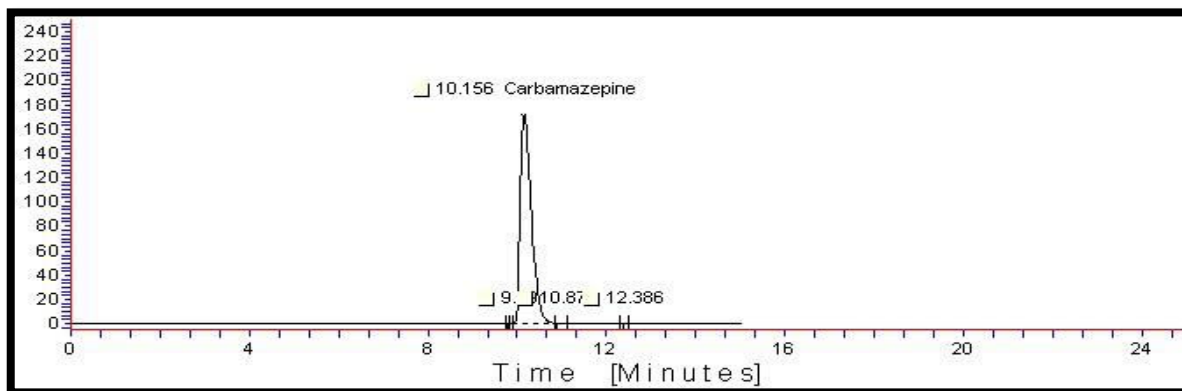
Fig.3: Chromatogram of Carbamazepine sample in alkali degradation
